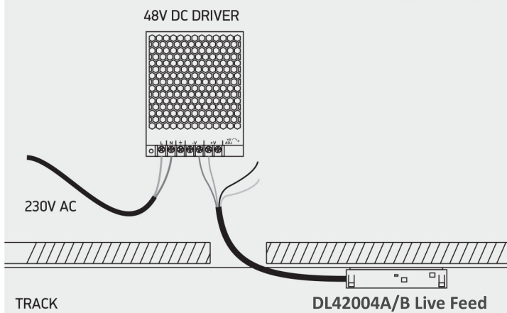
ON/OFF WIRING DIAGRAM
