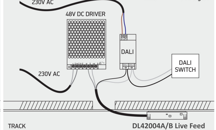
DALI WIRING DIAGRAM
